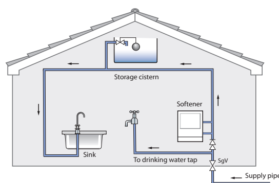
Fig 4: Connection for drinking tap upstream of the water softener.
